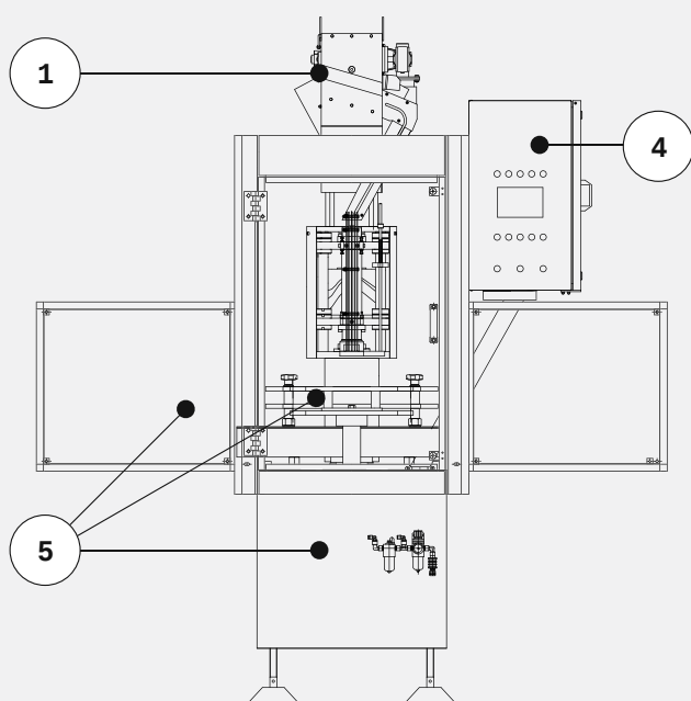
FREE STANDING EXECUTION
