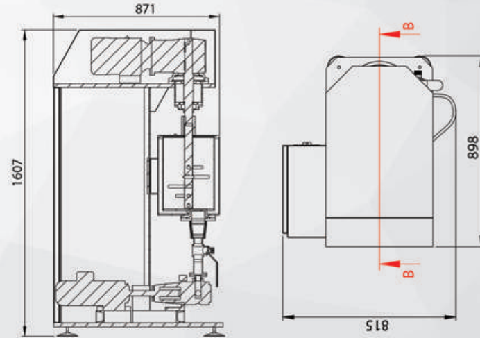
10 KG BİLYALI ÇİKOLATA MİKSERİ LAB TYPE BALL MILL REFINER - 10 KG
