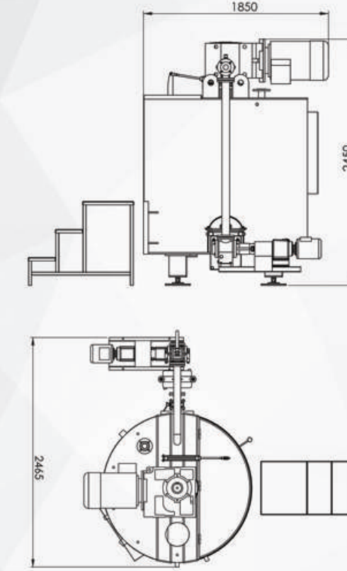
1000 KG BİLYALI ÇİKOLATA MİKSERİ LAB TYPE BALL MILL REFINER - 1000 KG
