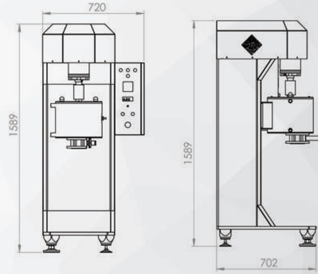
10 KG BİLYALI ÇİKOLATA MİKSERİ LAB TYPE BALL MILL REFINER - 10 KG
